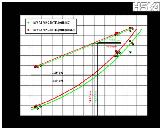
Figure 8: Full scale trial results without and with Mewis Duct®, AS VINCENTIA, power reduction: 6.5 % at contract speed 14.4 kts
