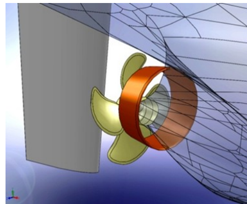
Figure 4: Mewis Duct®-Components, the pre-duct
