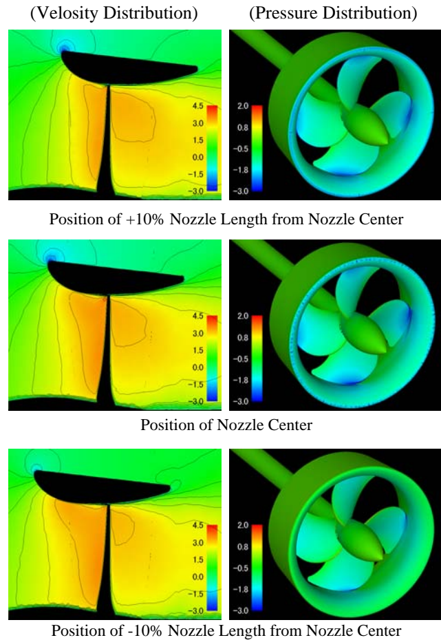
Figure 8 Comparison of Propeller Tip Position
