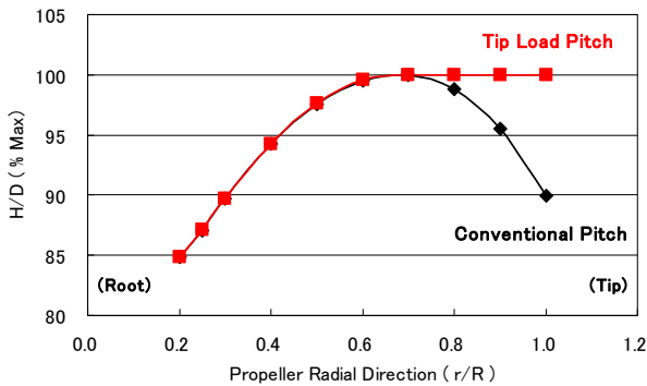
Figure 4 Propeller Pitch Distribution
