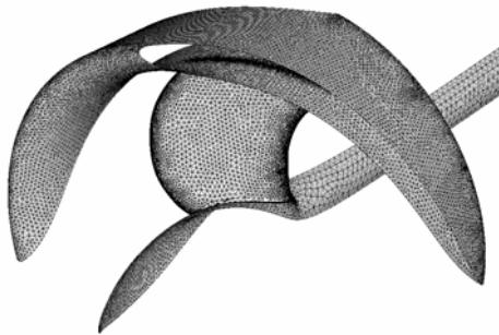
Figure 7 1/4 Cyclic Model for 3D Analysis
