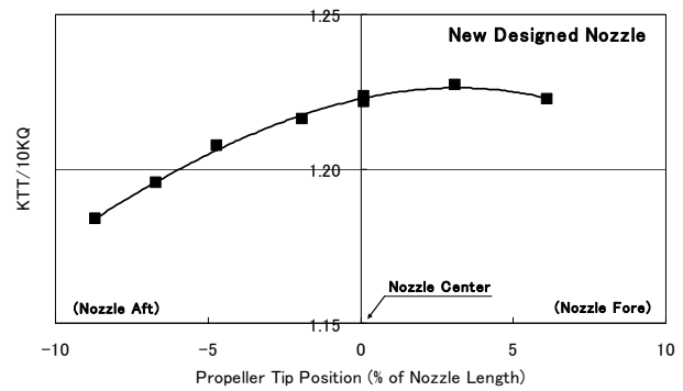
Figure 12 Model Test Results of Bollard Pull Efficiency
