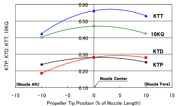
Figure 9 Calculation Results of Ducted Propeller Characteristics
