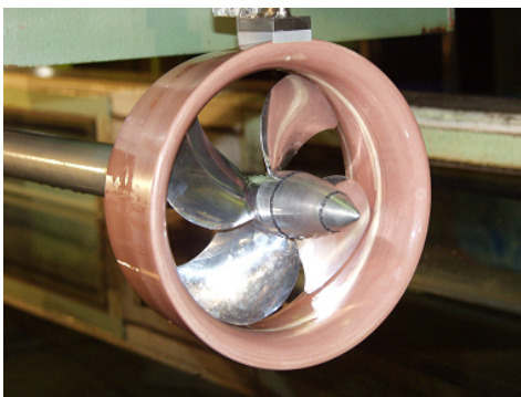
Figure 11 Model Ducted Propeller
