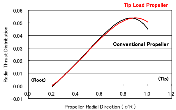
Figure 5 Radial Propeller Thrust Distribution
