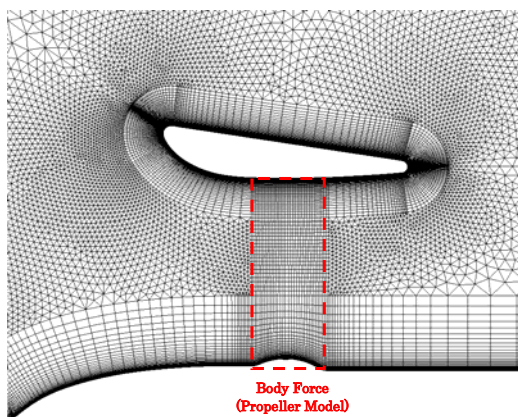
Figure 1 Calculation Meshes for 2D Analysis
