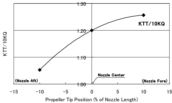
Figure 10 Calculation Results of Bollard Pull Efficiency
