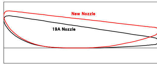
Figure 2 New Designed Nozzle Shape
