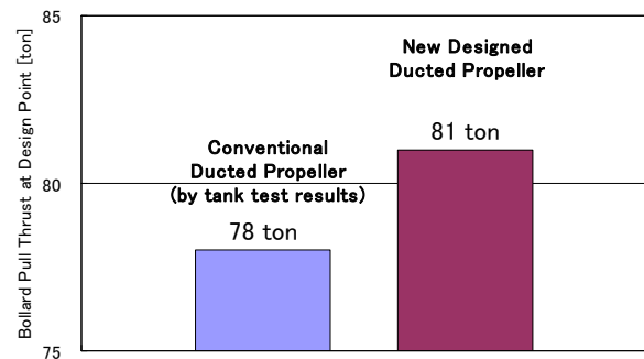
Figure 13 Comparison of Bollard Pull Thrust
